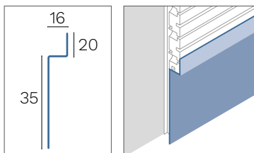
Profilo a C alluminio 8/10 C profile aluminum 8/10
