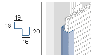
Profili a C alluminio 8/10 C profiles aluminum 8/10
