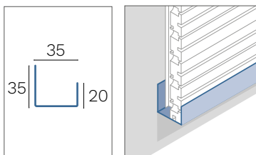
Profilo a M alluminio 8/10 M profile aluminum 8/10
