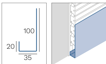
Profilo a F alluminio 8/10 F profile aluminum 8/10
