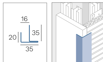
Profilo a C alluminio 8/10 C profile aluminum 8/10
